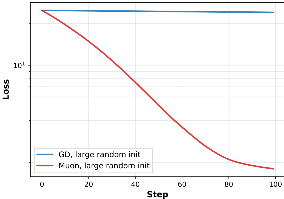
Loss: GD vs Muon (large random init)
